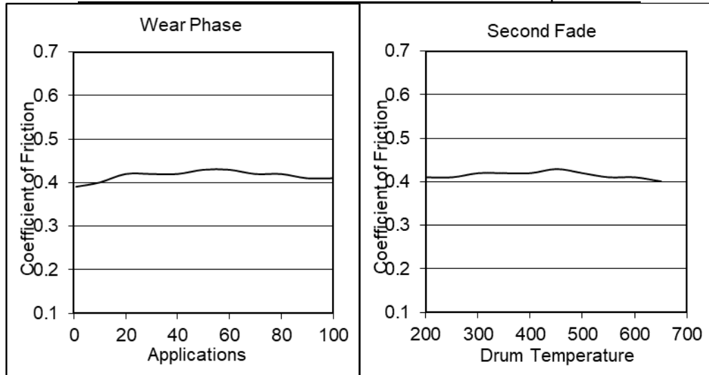
COEFFICIENT OF FRICTION from SAE J661a test procedure
